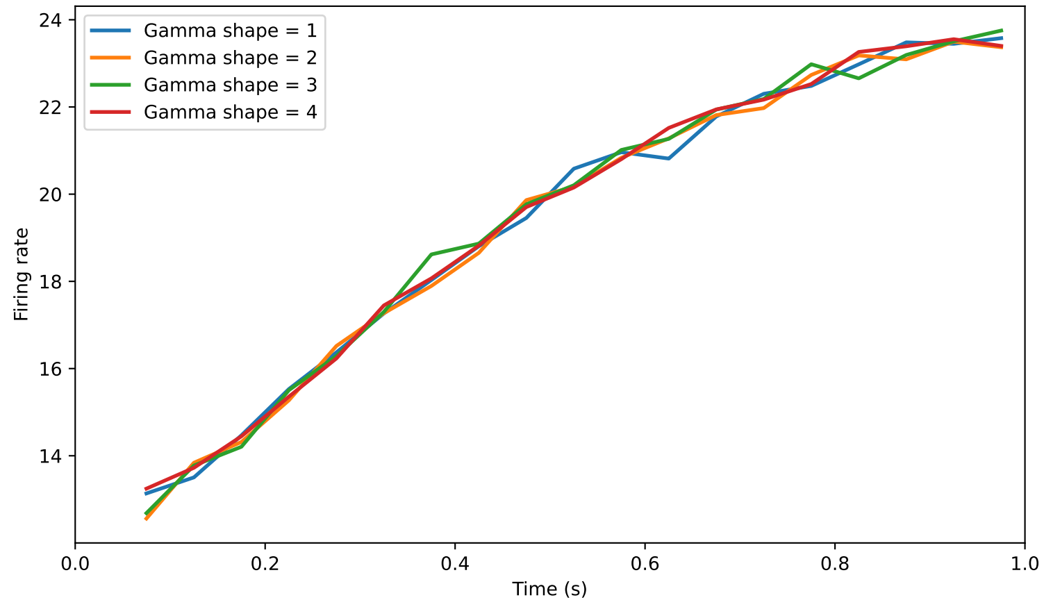
PSTH for step model: m = 50 , r = 2
